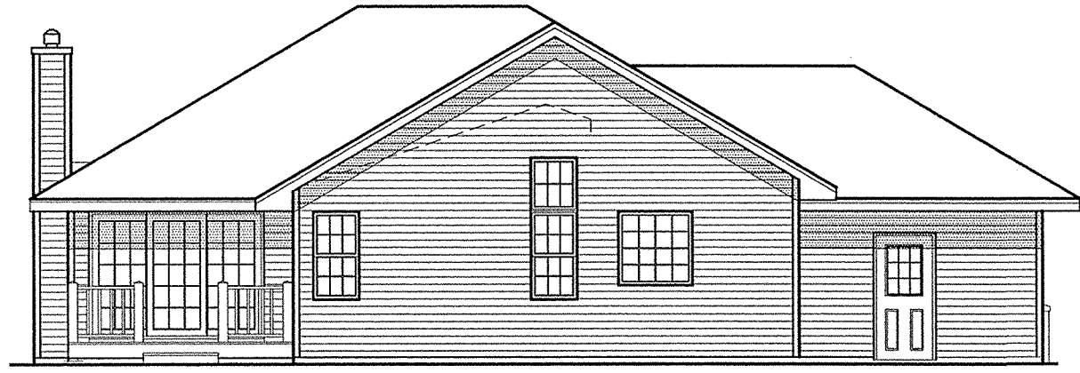
REAR ELEVATION
